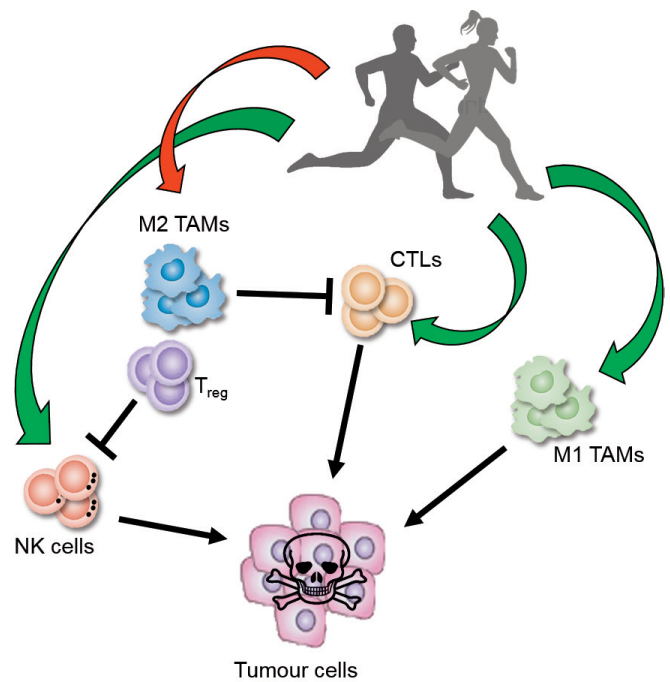
Figure 3: Overview of Exercise-Mediated Effects on the Immune Tumour Microenvironment.
