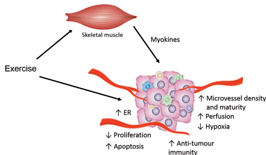
Figure 2: Proposed Mechanisms for the Effects of Exercise on the Tumour Microenvironment.
