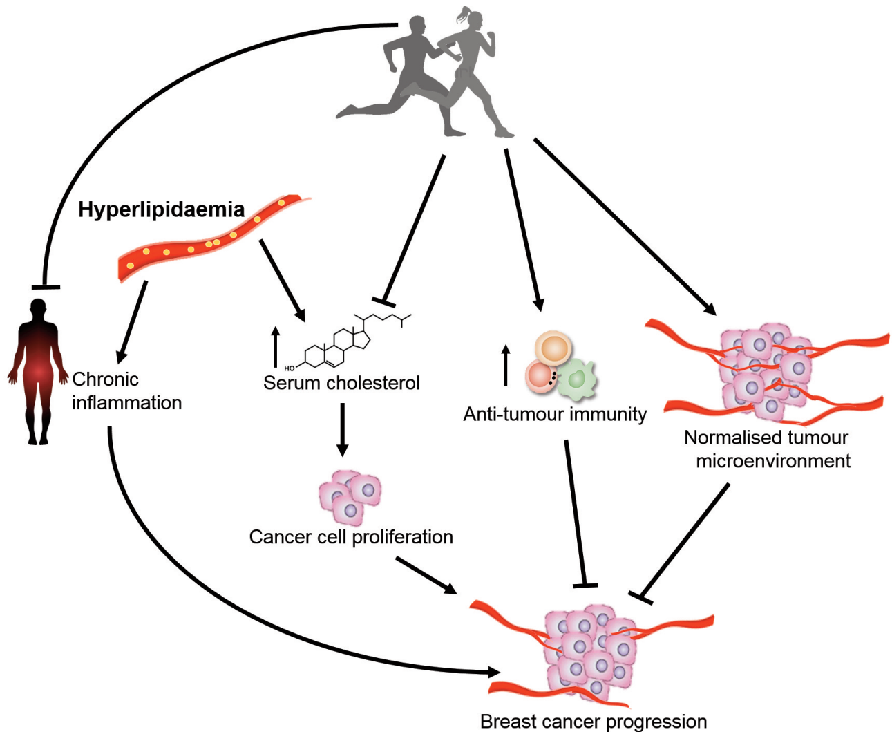
Figure 4: Hypothesised interplay of exercise and hyperlipidaemia in breast cancer progression.
