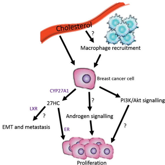
Figure 1: Potential Mechanisms of Cholesterol in Breast Cancer Progression.
